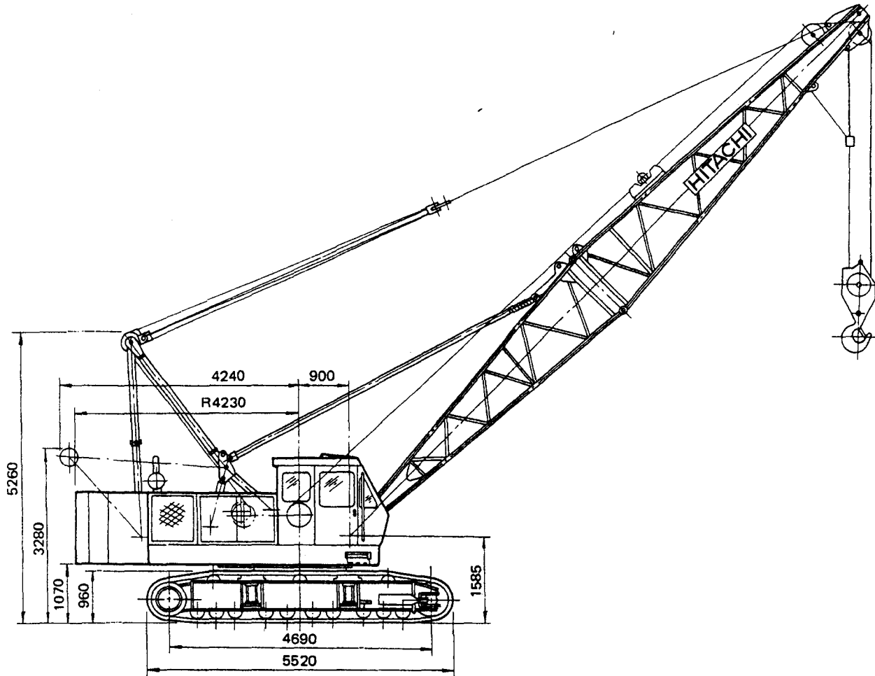
Working Range Figure of KH180-3 Crawler Crane
