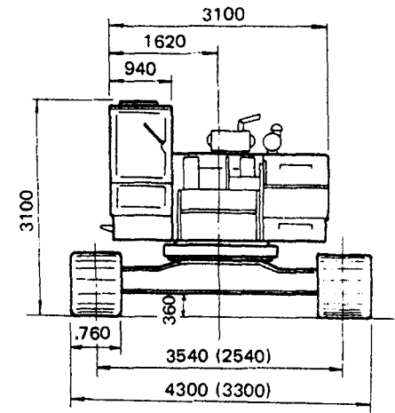
Dimension in parentheses ( ) are when the crawler is retracted.
